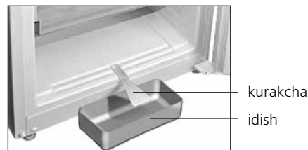
7 rasm — MBdan erigan suvni yig'ib olish
